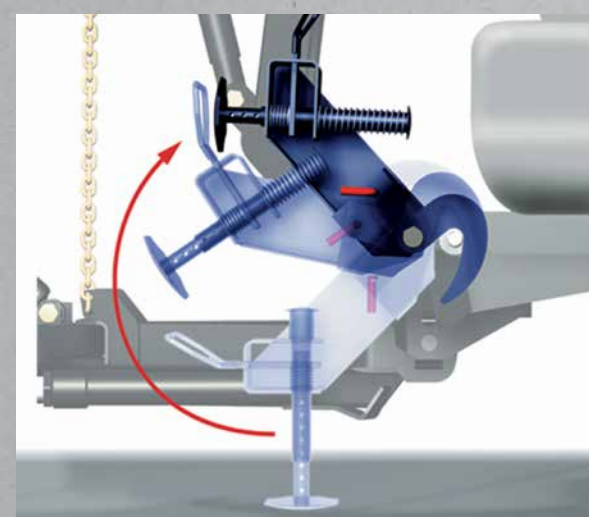
ATTACHMENT SYSTEMS Fast and easy installation and removal of the blade to keep you running.
