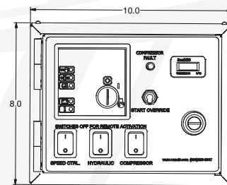
REMOTE PANEL
