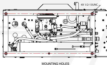
MOUNTING HOLES
