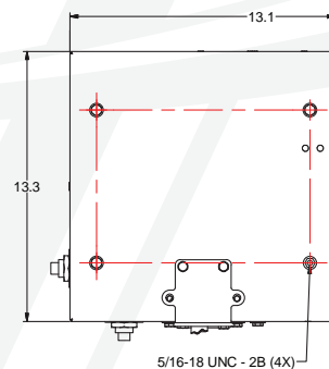
REMOTE PANEL WITHOUT OPTIONAL SPACER MOUNTING HOLES
