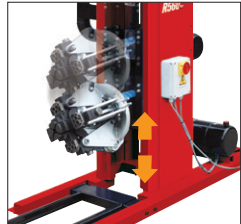
HYDRAULIC UP and DOWN MOVEMENT 4" minimum clamping 13" minimum height
