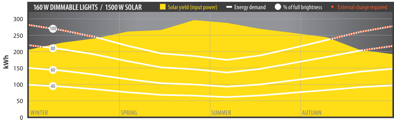
Programmable Solar Light Towers 1500-watt models
