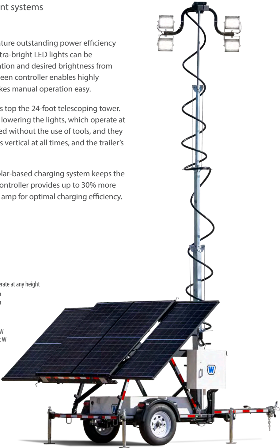
Programmable Solar Light Tower, 1500-watt Model WLTS-M-1500
