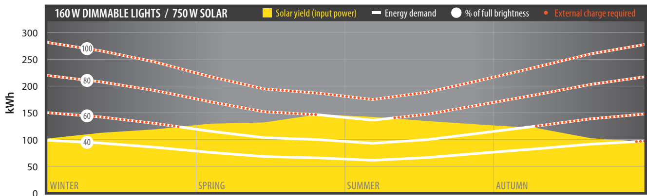
Programmable Solar Light Towers 750-watt model
