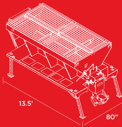
Retractable Legs
