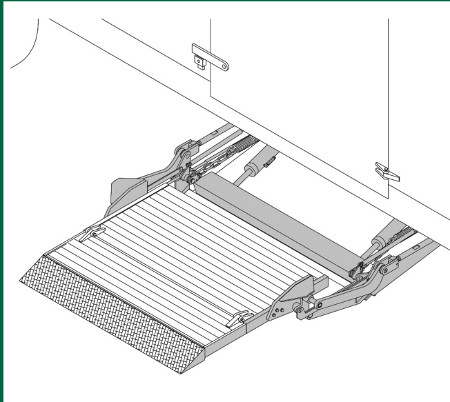
Platform in Loading/Unloading Position
