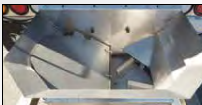
"Hex flow" chute and 24 inch spinner with adjustable baffles for optimal spread pattern
