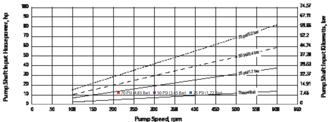
Horsepower Requirements
