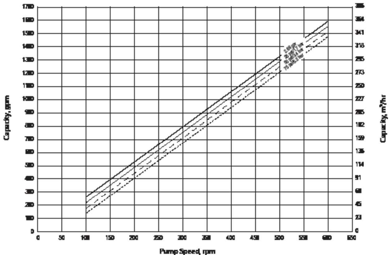
Performance Curve
