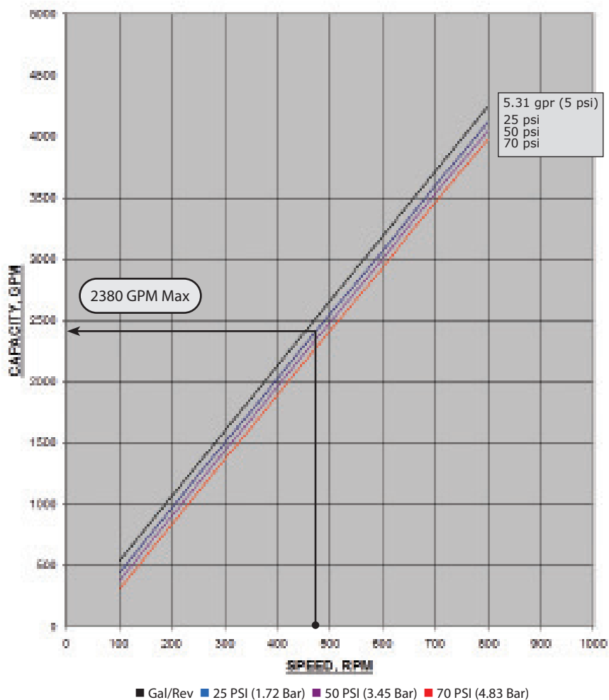
LobePro GL531d Performance Curve
