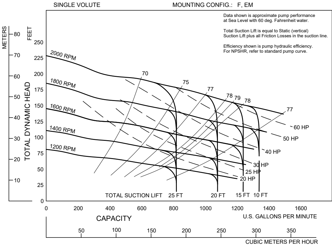
Performance Curve Model: PT6TPC-E75 Size: 6" (150mm) High Head Trash Pump
