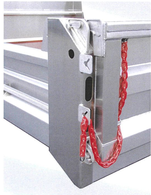
Pictured is a close view of the full-depth rear corner post with double chain adjusters and 10 gauge stainless steel rear bolster.
