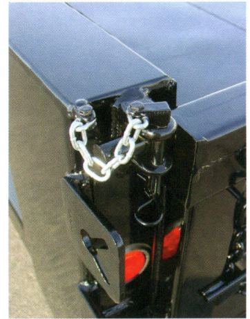
Double acting tailgate with drop pin upper hardware
