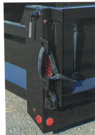
Screw Pin Top Release
