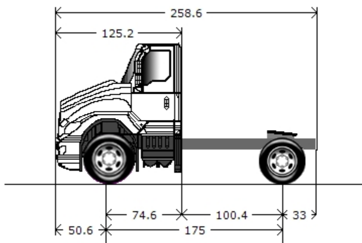
Model Profile 2022 LT625 4x2 (LT62A)
